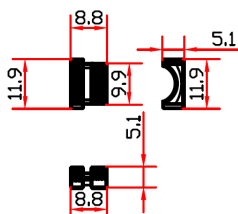
Strain Relief
